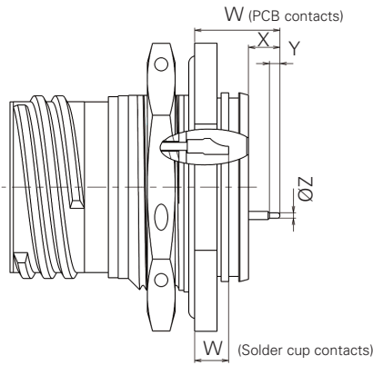
Type 23: Jam nut receptacle
