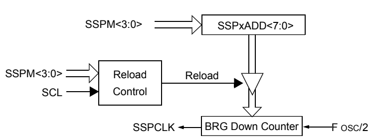
Figure 28-40. Baud Rate Generator Block Diagram
