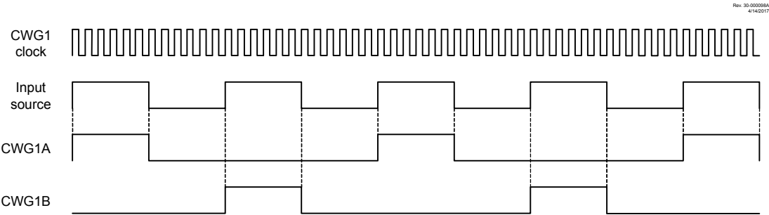
Figure 25-3. CWG Push-Pull Mode Operation
