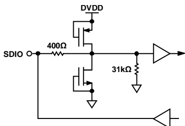
Figure 37. Equivalent SDIO Circuit
