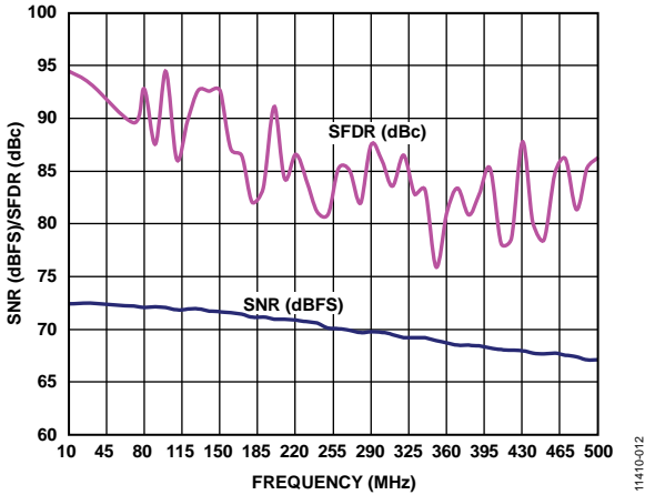
Figure 12. AD9683-170 Single-Tone SNR/SFDR vs. Input Frequency ( f_{IN} ), RFLCK = 680 MHz with Divide by 4 (Address 0x09 = 0x21)
